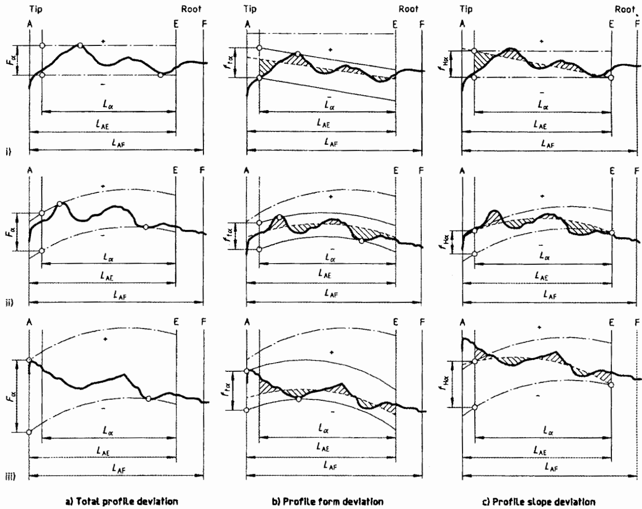
Figure 2 — Profile deviations
